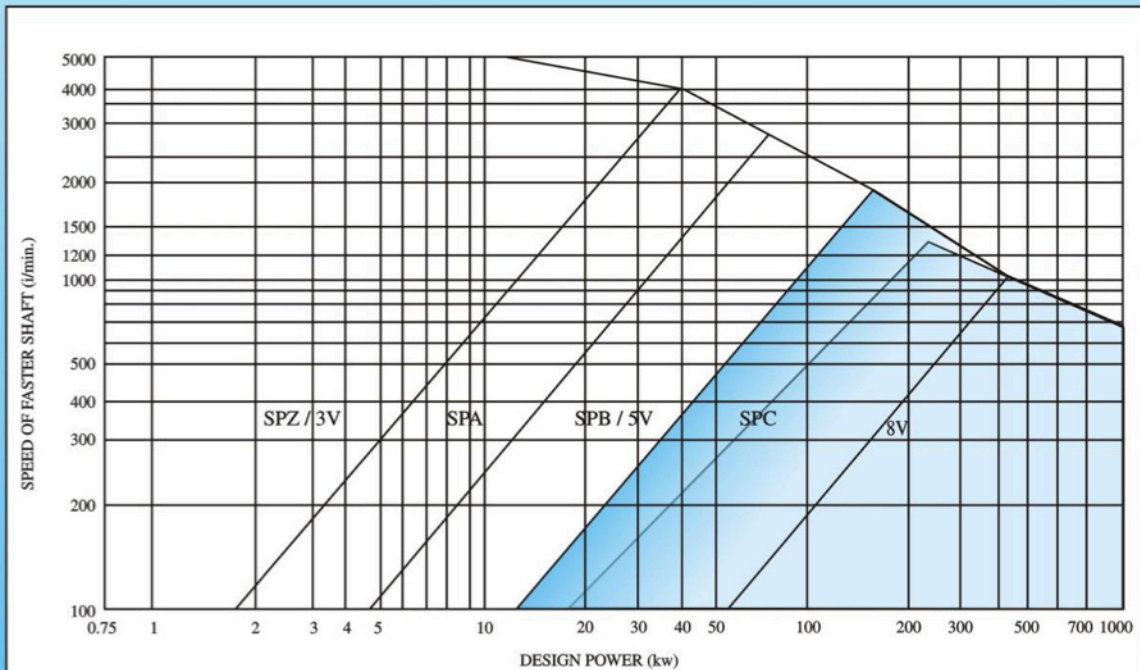
SELECTION OF WEDGE-/NARROW BELT CROSS SECTION
